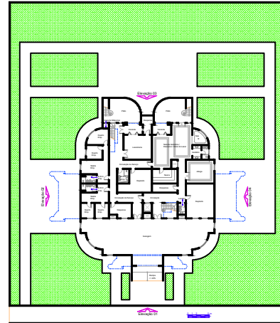
Subsolo A = 559,69 m 2
